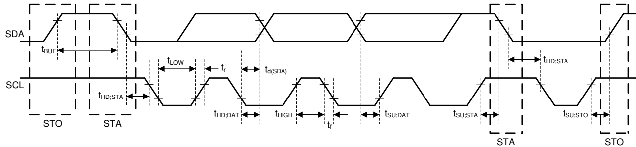
Figure 7-1. I²C Interface Timing Diagram
