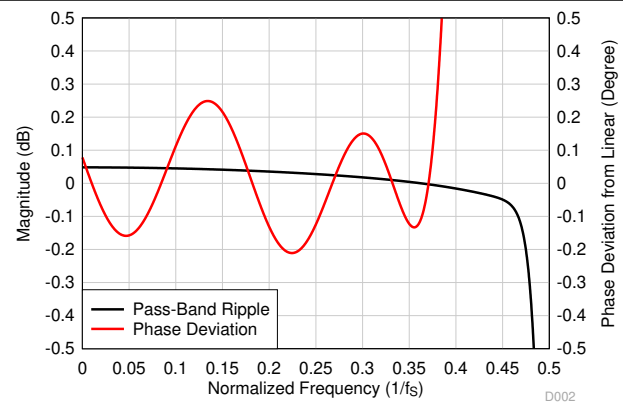
Figure 8-40. Low-Latency Decimation Filter Pass-Band Ripple and Phase Deviation
