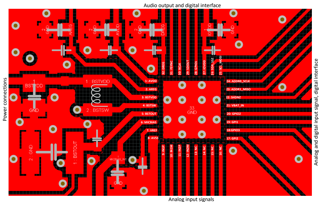
Figure 11-1. Layout Example of the PCM6020-Q1
