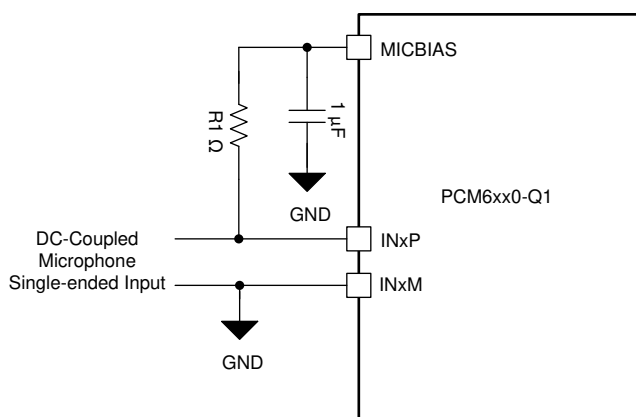
Figure 8-15. DC-Coupled Microphone Single-Ended Input Connection
