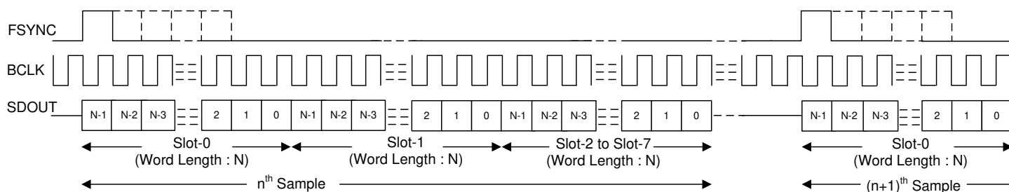
Figure 8-4. TDM Mode Protocol Timing (TX_OFFSET = 0 and BCLK_POL = 1)
