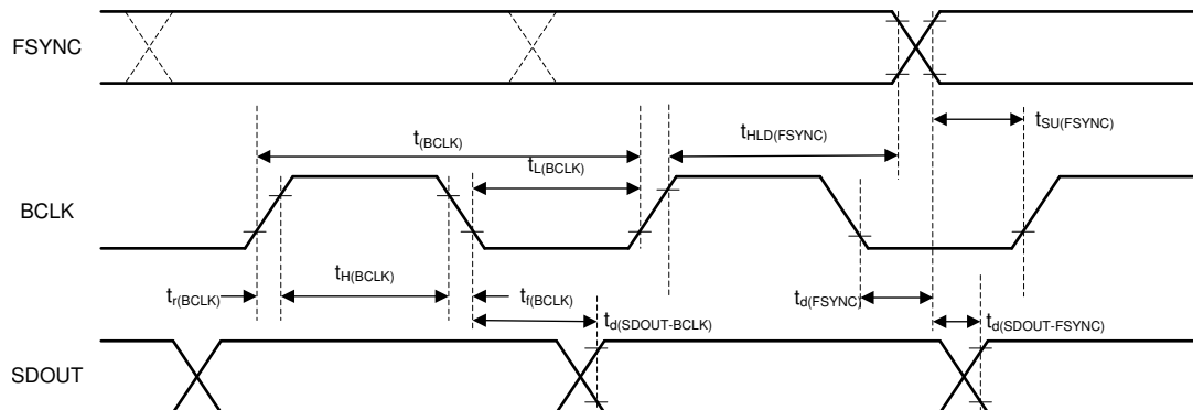
Figure 7-3. TDM, I²S, LJ Interface Timing Diagram
