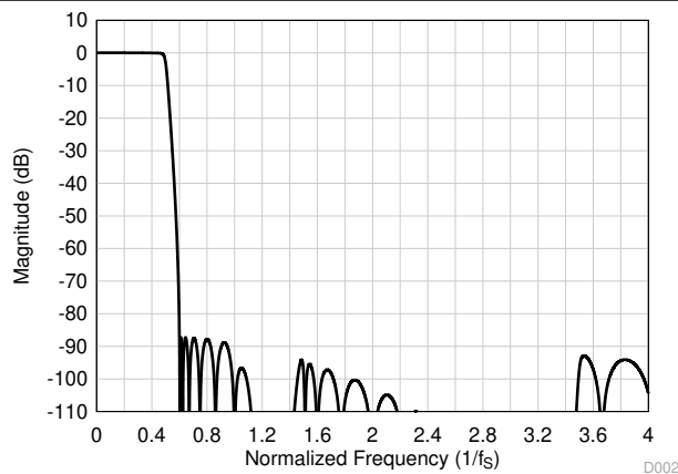
Figure 8-39. Low-Latency Decimation Filter Magnitude Response
