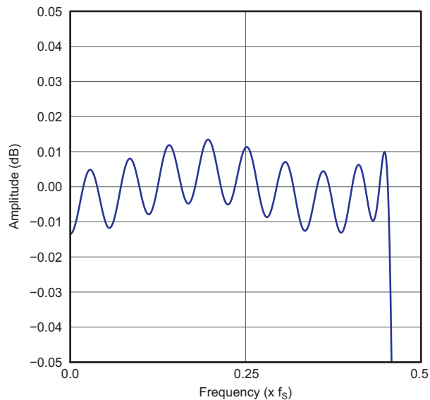
Figure 27. Normal x4 Interpolation Filter Passband Ripple
