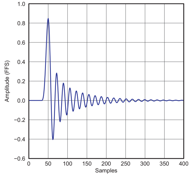
Figure 32. Low Latency x8 Interpolation Filter Impulse Response
