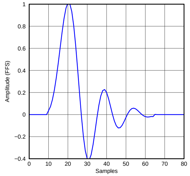
Figure 41. Asymmetric FIR x8 Interpolation Filter Impulse Response, Single Rate
