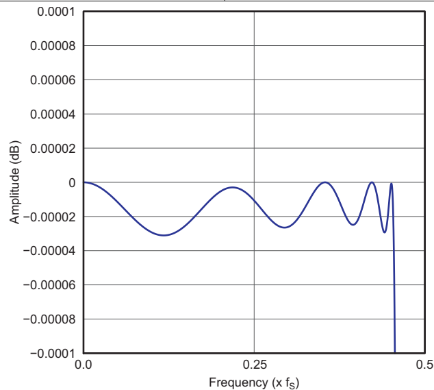
Figure 39. Low Latency x2 Interpolation Filter Passband Ripple
