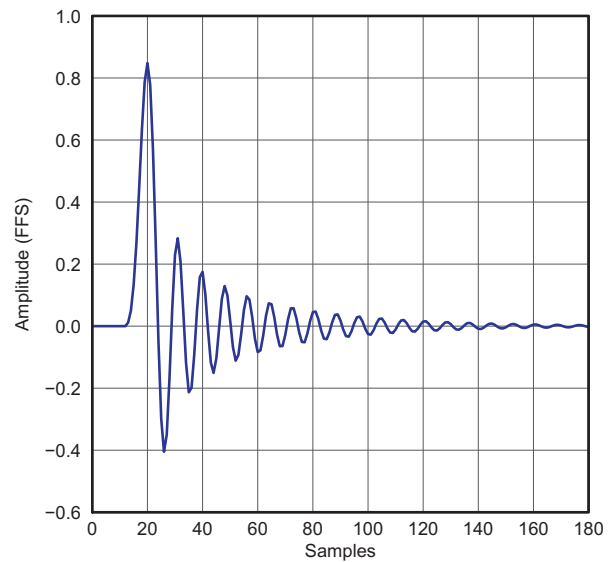
Figure 35. Low Latency x4 Interpolation Filter Impulse Response
