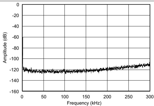
Figure 14. FFT Plot at BPZ With Analog Mute (AMUTE)
