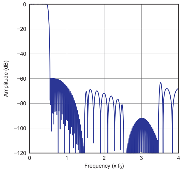
Figure 22. Normal x8 Interpolation Filter Frequency Response
