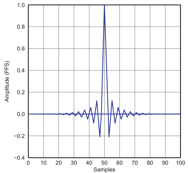
Figure 29. Normal x2 Interpolation Filter Impulse Response
