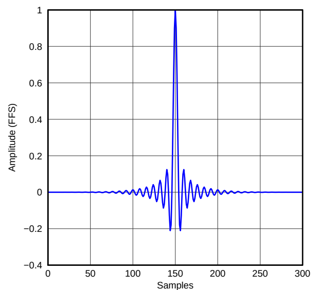
Figure 53. High-Attenuation x4 Interpolation Filter Impulse Response, Dual Rate
