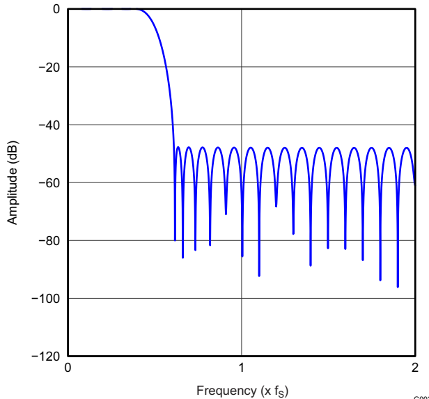
Figure 43. Asymmetric FIR x4 Interpolation Filter Frequency Response, Dual Rate
