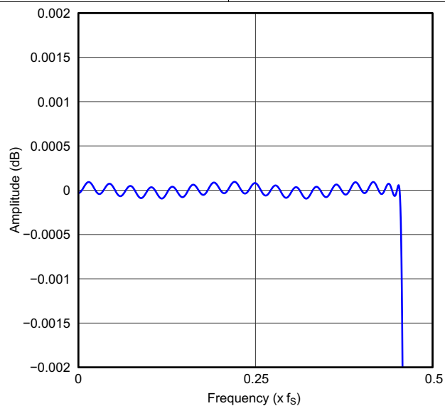
Figure 54. High-Attenuation x4 Interpolation Filter Passband Ripple, Dual Rate
