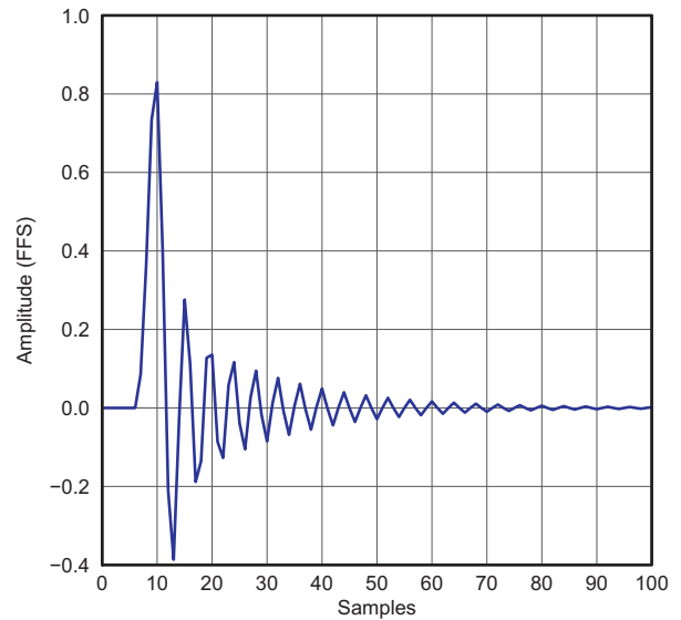
Figure 38. Low Latency x2 Interpolation Filter Impulse Response
