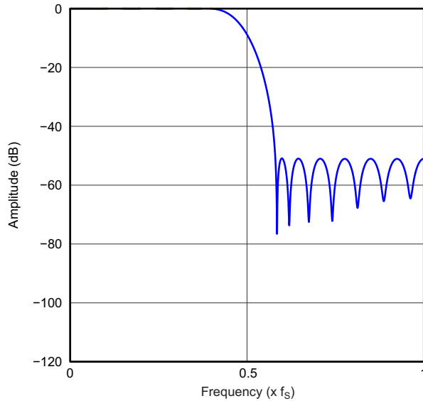
Figure 46. Asymmetric FIR x2 Interpolation Filter Frequency Response, Quad Rate
