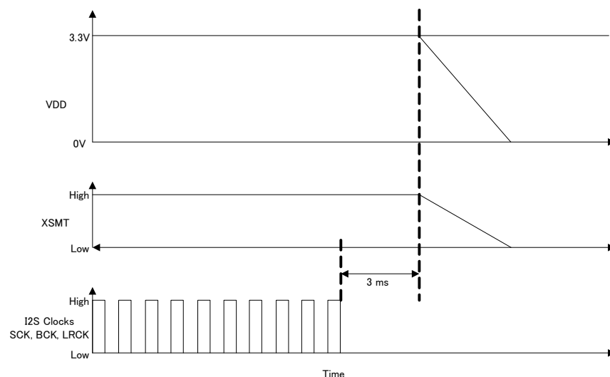
Figure 77. Stop I²C Clocks
