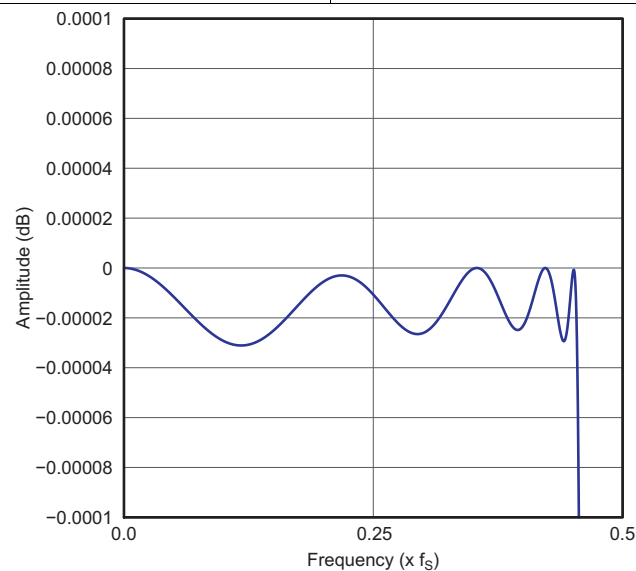
Figure 36. Low Latency x4 Interpolation Filter Passband Ripple
