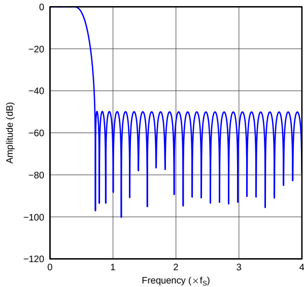
Figure 40. Asymmetric FIR x8 Interpolation Filter Frequency Response, Single Rate
