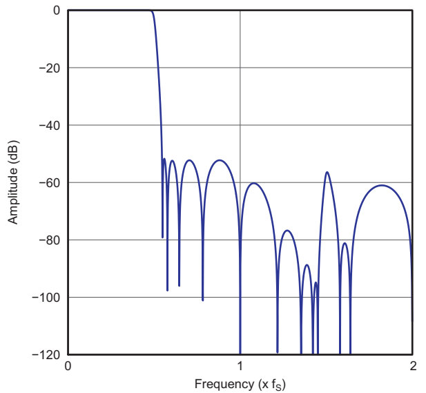
Figure 34. Low Latency x4 Interpolation Filter Frequency Response
