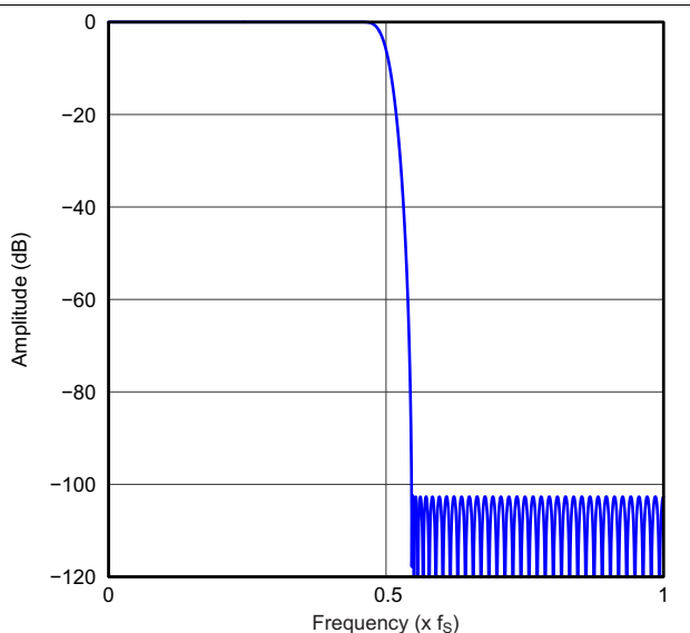
Figure 55. High-Attenuation x2 Interpolation Filter Frequency Response, Quad Rate
