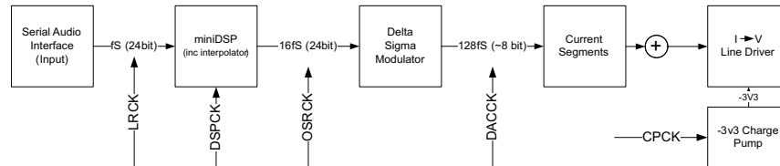
Figure 60. Audio Flow with Respective Clocks
