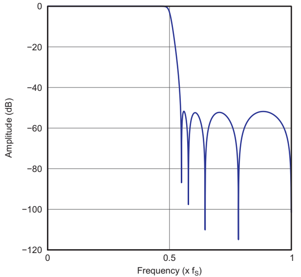
Figure 37. Low Latency x2 Interpolation Filter Frequency Response
