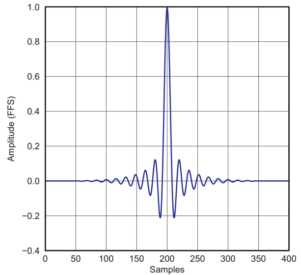
Figure 23. Normal x8 Interpolation Filter Impulse Response
