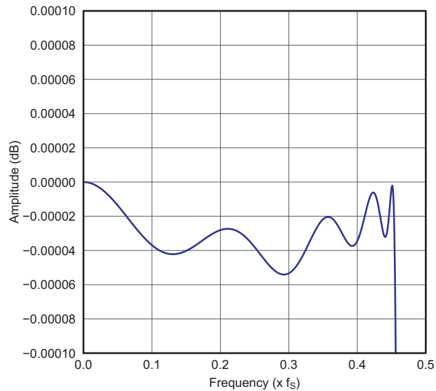
Figure 33. Low Latency x8 Interpolation Filter Passband Ripple
