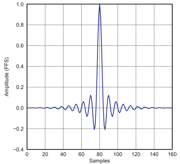
Figure 26. Normal x4 Interpolation Filter Impulse Response
