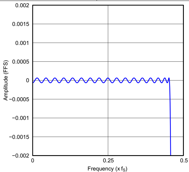
Figure 57. High-Attenuation x2 Interpolation Filter Passband Ripple, Quad Rate
