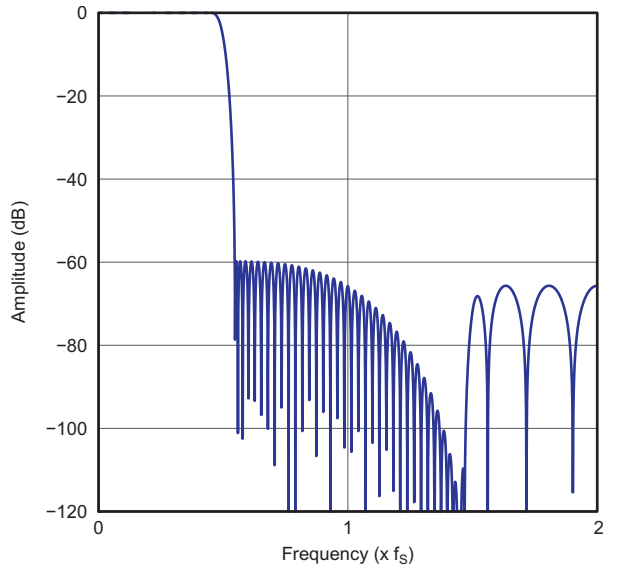
Figure 25. Normal x4 Interpolation Filter Frequency Response
