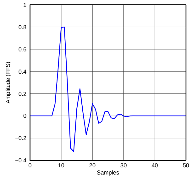
Figure 47. Asymmetric FIR x2 Interpolation Filter Impulse Response, Quad Rate
