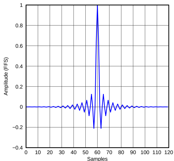
Figure 56. High-Attenuation x2 Interpolation Filter Impulse Response, Quad Rate
