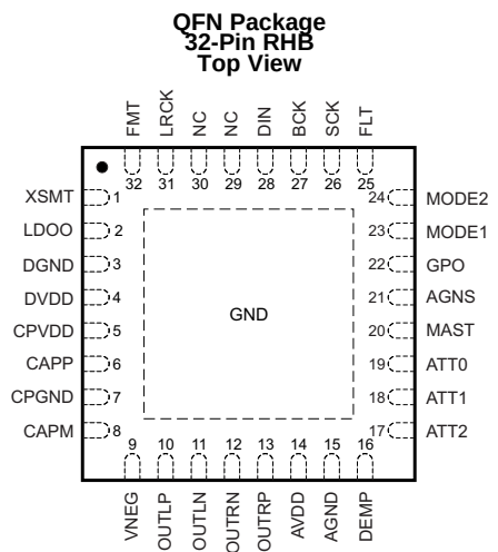
Figure 3. Hardware Control
