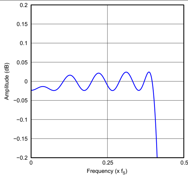
Figure 48. Asymmetric x2 Interpolation Filter Passband Ripple, Quad Rate
