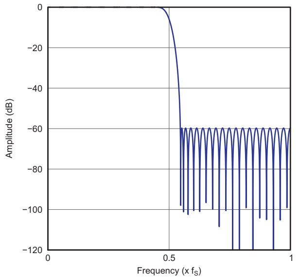
Figure 28. Normal x2 Interpolation Filter Frequency Response
