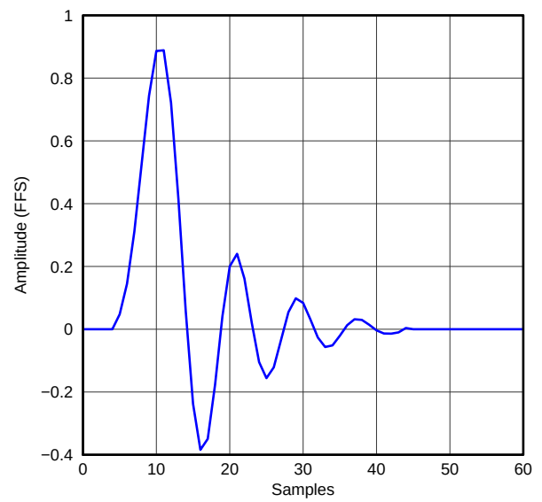
Figure 44. Asymmetric FIR x4 Interpolation Filter Impulse Response, Dual Rate
