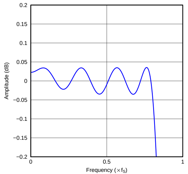
Figure 45. Asymmetric x4 Interpolation Filter Passband Ripple, Dual Rate
