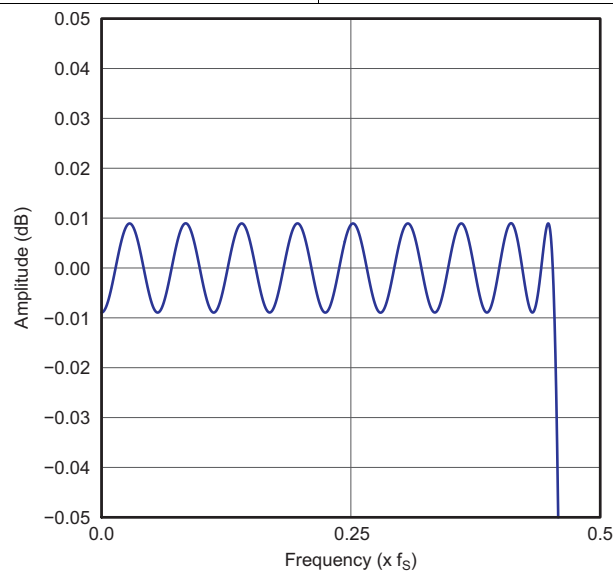
Figure 30. Normal x2 Interpolation Filter Passband Ripple
