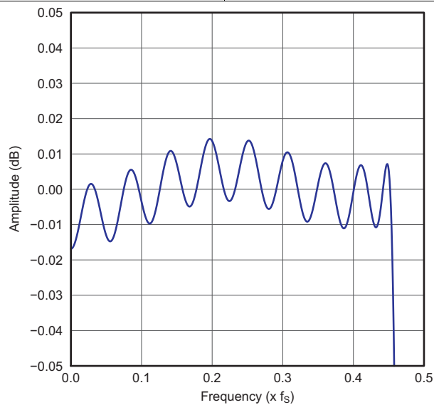
Figure 24. Normal x8 Interpolation Filter Passband Ripple
