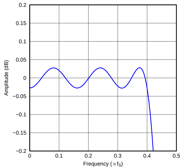
Figure 42. Asymmetric FIR x8 Interpolation Filter Passband Ripple, Single Rate
