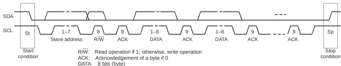
Figure 71. Packet Protocol
