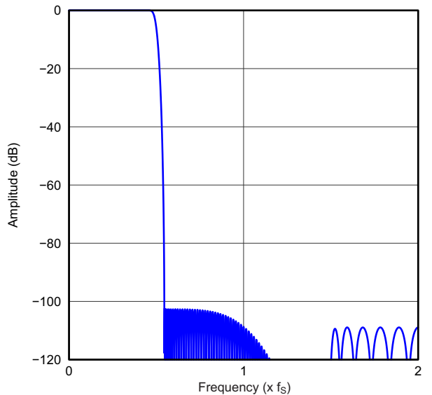
Figure 52. High-Attenuation x4 Interpolation Filter Frequency Response, Dual Rate
