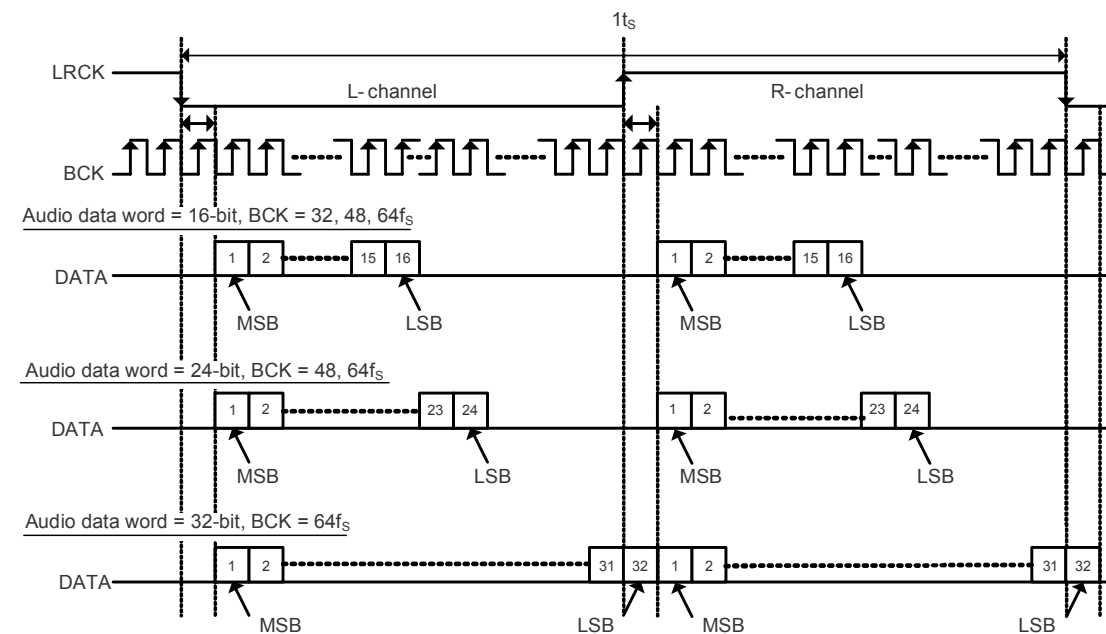
Figure 16. I²S Audio Data Format
