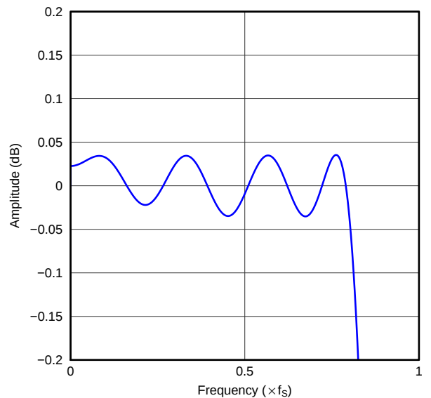
Figure 44. Asymmetric x4 Interpolation Filter Passband Ripple, Dual Rate
