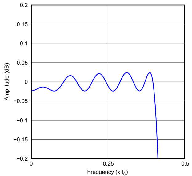
Figure 47. Asymmetric x2 Interpolation Filter Passband Ripple, Quad Rate
