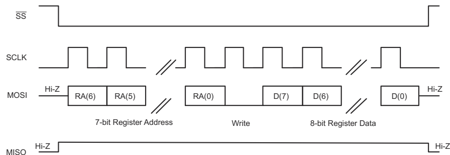
Figure 7-71. SPI Single-Byte Write Transfer
