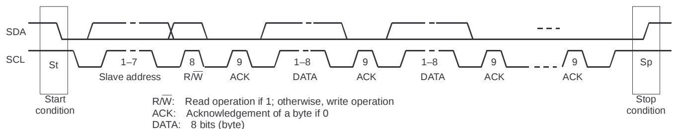
Figure 73. Packet Protocol
