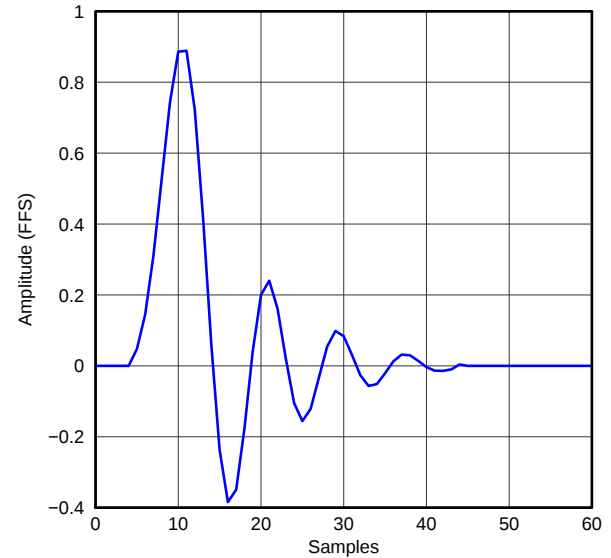
Figure 41. Asymmetric FIR x4 Interpolation Filter Impulse Response, Dual Rate
