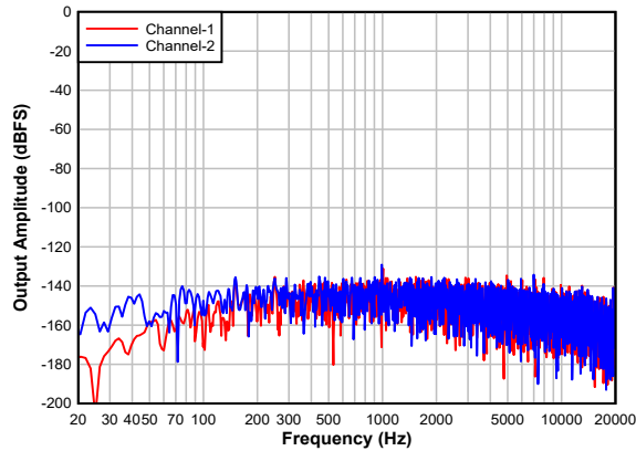
Figure 7-22. Single Ended FFT With Idle Input With DRE Enabled
