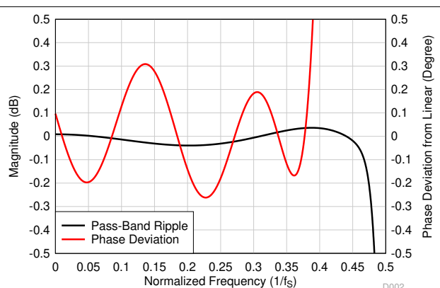
Figure 8-42. Low-Latency Decimation Filter Pass-Band Ripple and Phase Deviation
