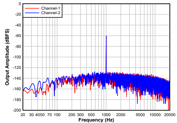
Figure 7-25. Single Ended FFT With a -60-dBr Input With DRE Disabled
