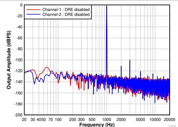
Figure 7-27. Differential FFT With a -1-dBr Input With DRE Disabled
