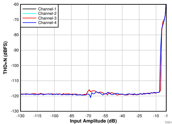
Figure 7-28. PDM Input THD+N vs Input Amplitude
