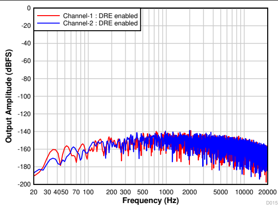
Figure 7-18. Differential FFT With Idle Input With DRE Enabled
