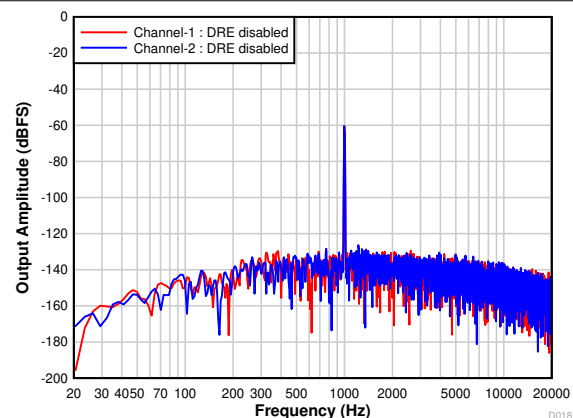
Figure 7-21. Differential FFT With a -60-dBr Input With DRE Disabled
