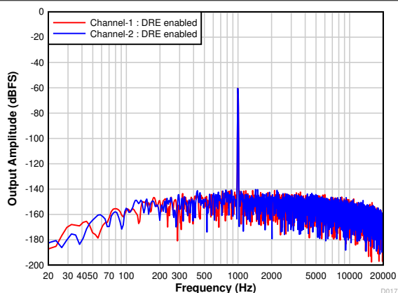
Figure 7-20. Differential FFT With a -60-dBr Input With DRE Enabled
