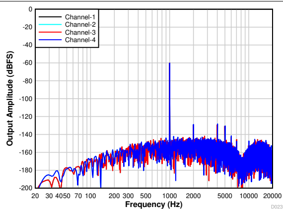
Figure 7-30. PDM Input FFT With a -60-dBr Input
