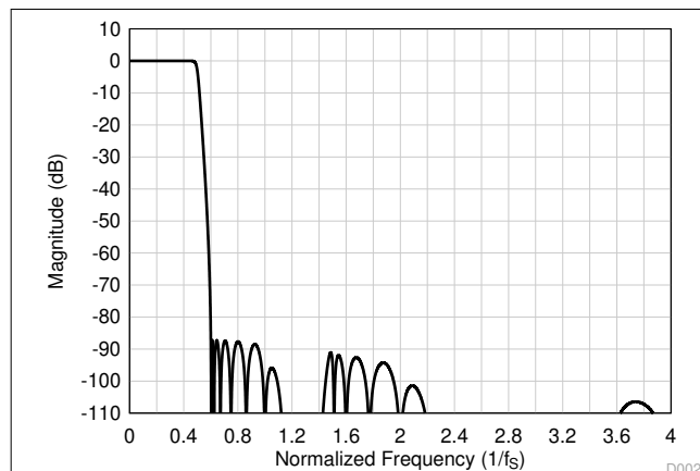
Figure 8-39. Low-Latency Decimation Filter Magnitude Response
