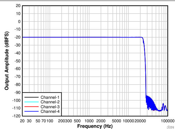
Figure 7-31. PDM Input Frequency Response With a -20-dBr Input
