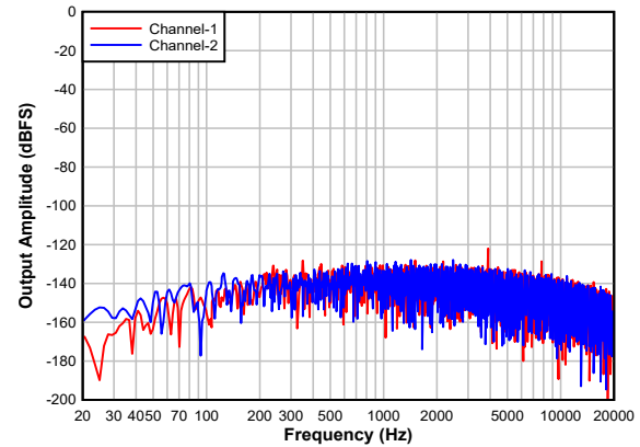
Figure 7-23. Single Ended FFT With Idle Input With DRE Disabled
