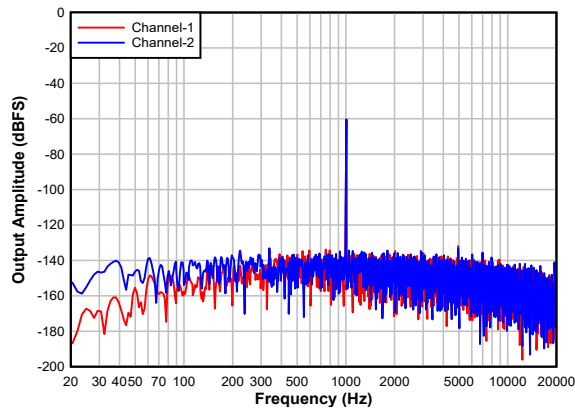
Figure 7-24. Single Ended FFT With a -60-dBr Input With DRE Enabled
