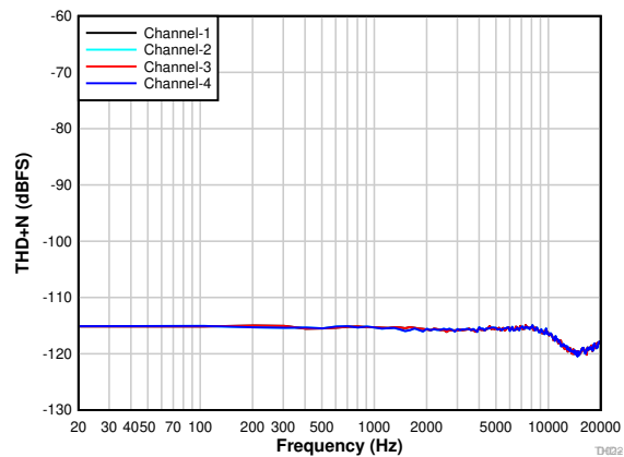
Figure 7-29. PDM Input THD+N vs Input Frequency With a -20-dBr Input
