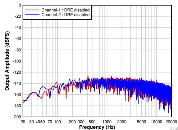
Figure 7-19. Differential FFT With Idle Input With DRE Disabled
