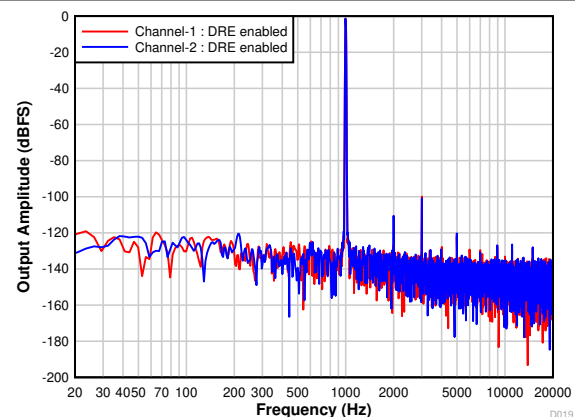
Figure 7-26. Differential FFT With a -1-dBr Input With DRE Enabled
