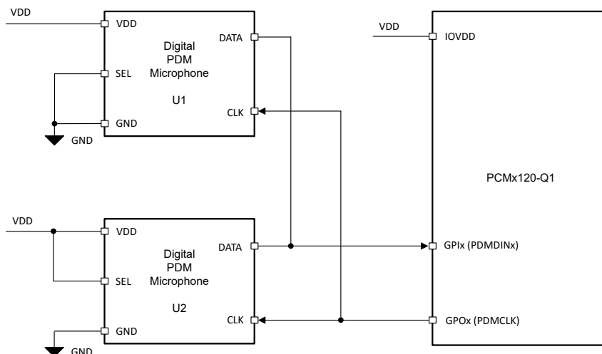
Figure 8-64. Digital PDM Microphones Connection Diagram for the PCM5120-Q1
