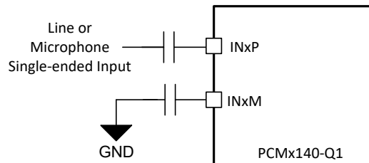
Figure 7-15. Single-Ended AC-Coupled Input Connection
