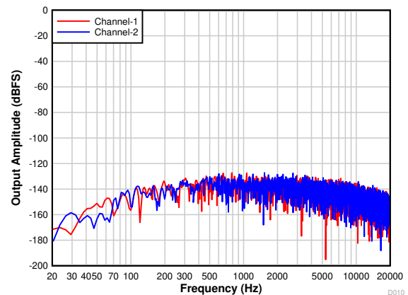
Figure 7-13. Differential FFT With Idle Input
