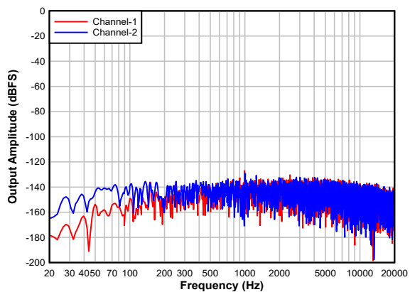
Figure 7-15. Single Ended FFT With Idle Input
