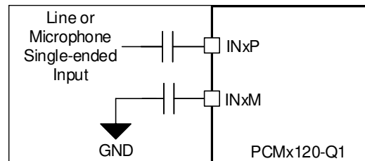
Figure 8-15. Single-Ended, AC-Coupled Input Connection
