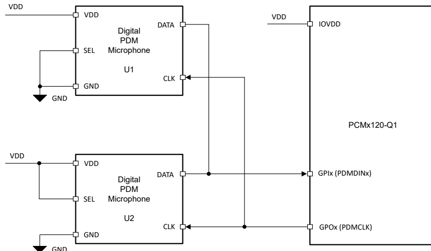
Figure 8-64. Digital PDM Microphones Connection Diagram for the PCM3120-Q1
