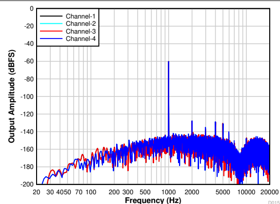
Figure 7-20. PDM Input FFT With a -60-dBr Input
