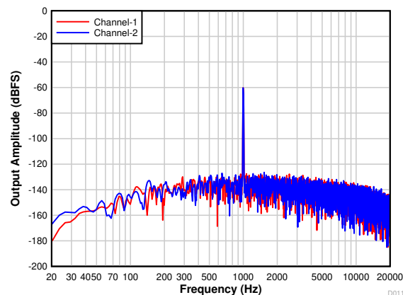
Figure 7-14. Differential FFT With a -60-dBr Input
