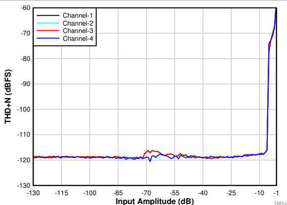
Figure 7-18. PDM Input THD+N vs Input Amplitude
