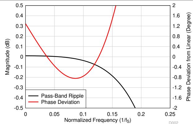
Figure 8-62. Ultra-Low-Latency Decimation Filter Pass-Band Ripple and Phase Deviation
