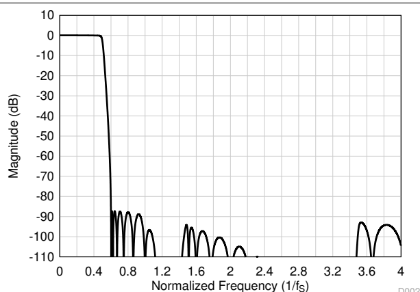
Figure 8-37. Low-Latency Decimation Filter Magnitude Response
