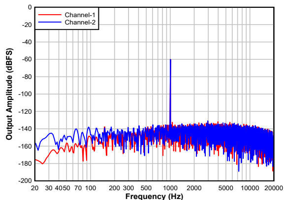
Figure 7-16. Single Ended FFT With a -60-dBr Input
