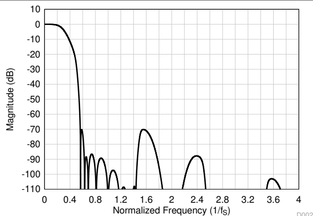
Figure 8-61. Ultra-Low-Latency Decimation Filter Magnitude Response
