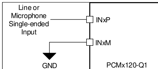
Figure 8-14. Single-Ended, DC-Coupled Input Connection
