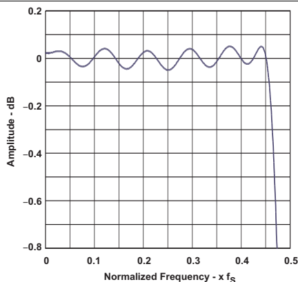
Figure 3. Passband Ripple
