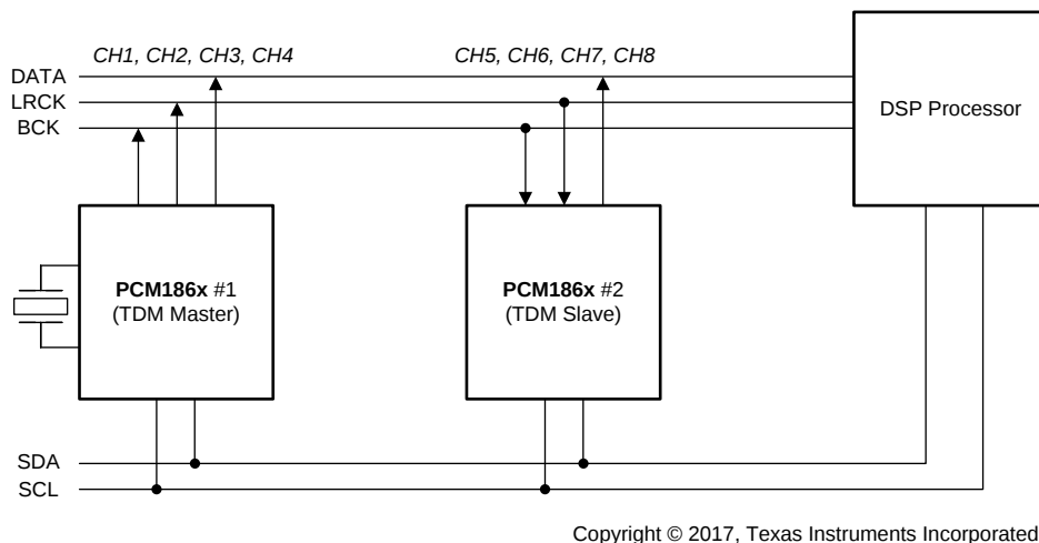
Figure 59. TDM With Two PCM186x
