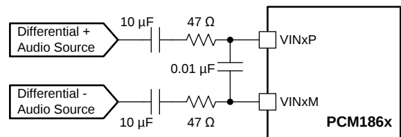
Figure 63. Differential Input Circuit With Additional AntiAliasing Filter
