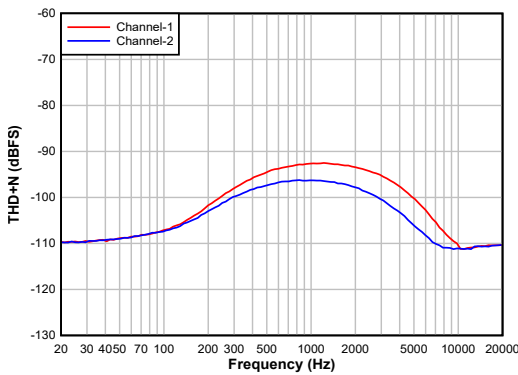
Figure 7-5. Differential Input: THD+N vs Input Frequency With a -1-dBr Input
