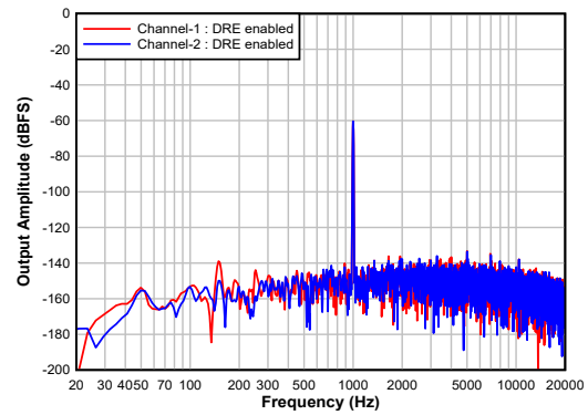
Figure 7-20. Single-ended Input: FFT With a -60-dBr Input and DRE Enabled
