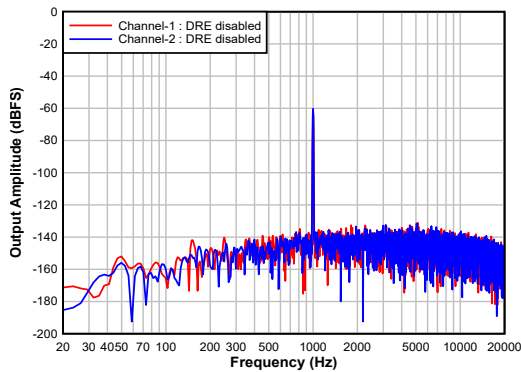
Figure 7-21. Single-ended Input: FFT With a -60-dBr Input and DRE Disabled
