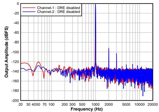
Figure 7-22. Single-ended Input: FFT With a -1-dBr Input
