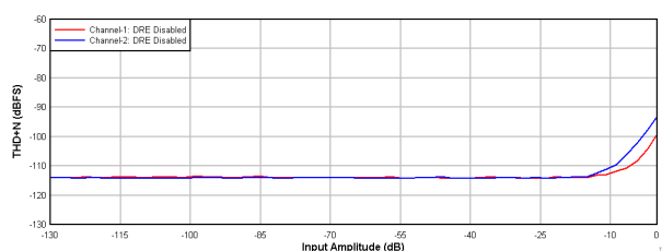
Figure 9-5. PCM1820-Q1: THD+N vs Input Amplitude With DRE Disabled
