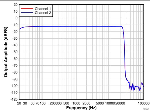
Figure 7-6. PCM1820-Q1: Frequency Response With a -12-dBr Input
