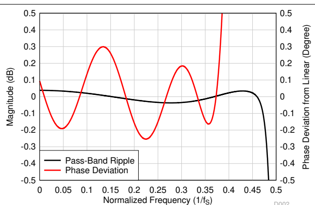
Figure 8-32. Low-Latency Decimation Filter Pass-Band Ripple and Phase Deviation
