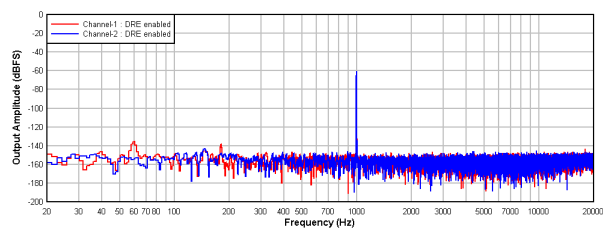
Figure 9-2. PCM1820-Q1: FFT With a -60-dBr Input With DRE Enabled
