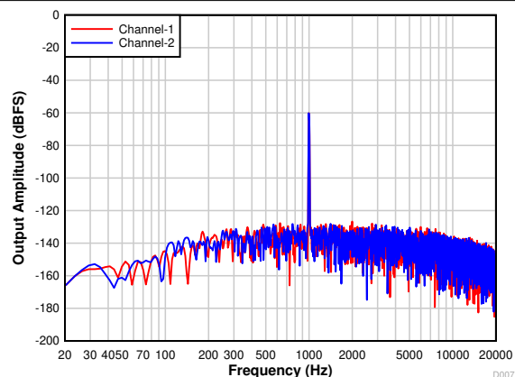
Figure 7-19. PCM1821-Q1: FFT With a -60\text{-dBr} Input and DRE Enabled
