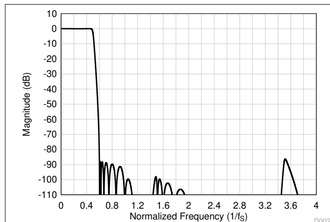
Figure 8-31. Low-Latency Decimation Filter Magnitude Response
