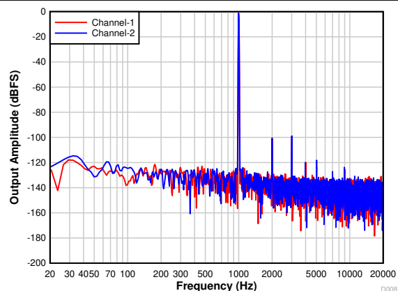
Figure 7-20. PCM1821: FFT With a -1\text{-dBr} Input
