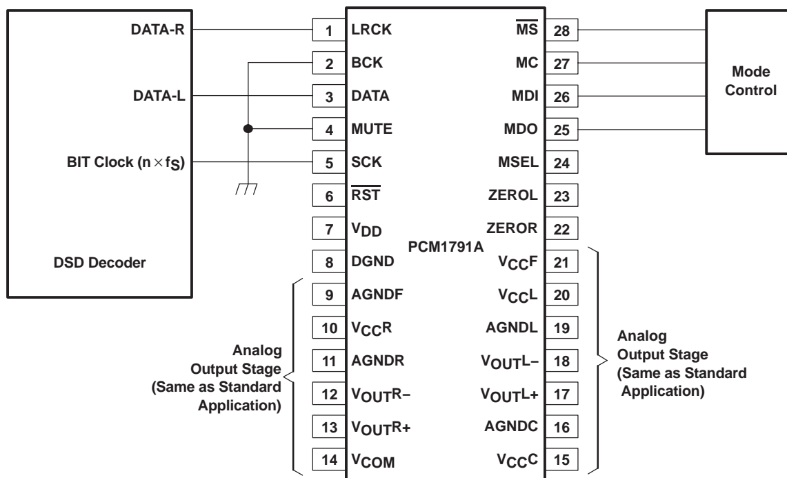
Figure 41. Connection Diagram in DSD Mode
