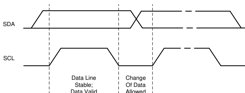
Figure 7-4. Bit Transfer
