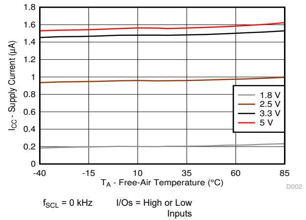
Figure 5-2. Supply Current ( I_{\text{CC}} , Standby Mode) vs Temperature ( T_A ) at Four Supply Voltages
