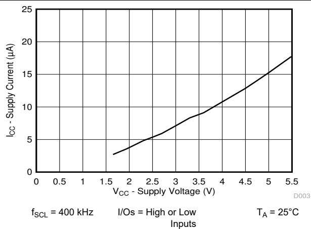
Figure 5-3. Supply Current ( I_{\text{CC}} , Operating Mode) vs Supply Voltage ( V_{\text{CC}} )
