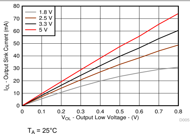
Figure 5-5. Sink Current ( I_{\text{OL}} ) vs Output Low Voltage ( V_{\text{OL}} ) for P-Ports at Four Supply Voltages
