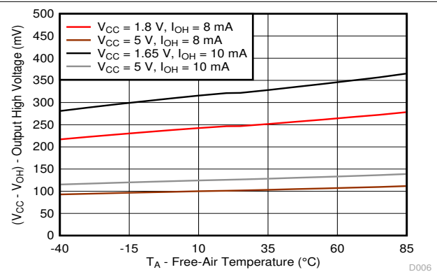
Figure 5-6. Output High Voltage ( V_{\text{CC}} - V_{\text{OH}} ) vs Temperature ( T_A ) for P-Ports
