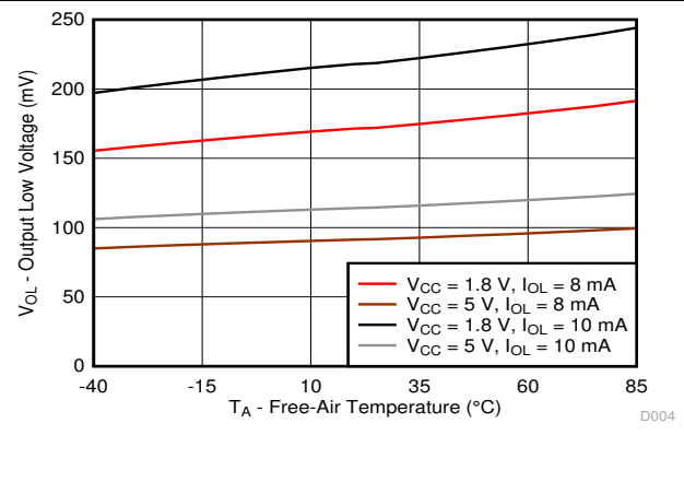
Figure 5-4. Output Low Voltage ( V_{\text{OL}} ) vs Temperature ( T_A ) for P-Port I/Os
