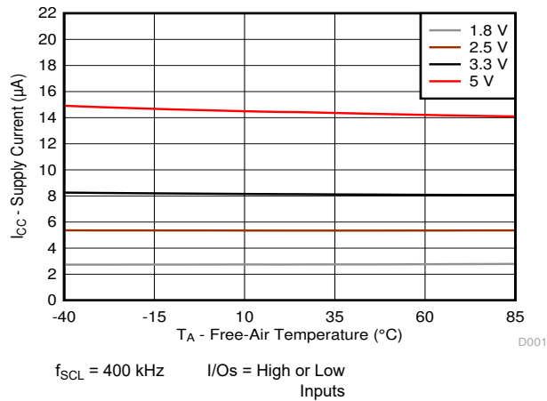
Figure 5-1. Supply Current ( I_{\text{CC}} , Operating Mode) vs Temperature ( T_A ) at Four Supply Voltages
