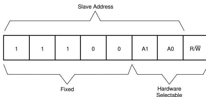
Figure 7-6. PCA9538 Address
