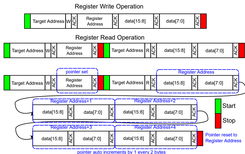
Figure 8-8. I²C Operations
