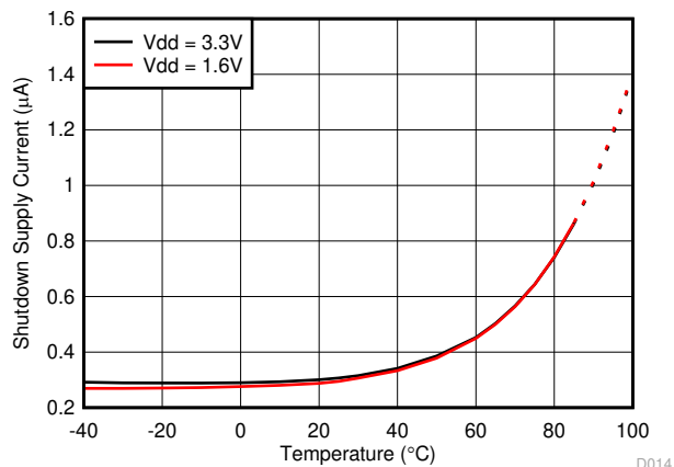
Figure 7-18. Shutdown Current vs Temperature
