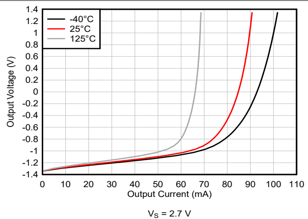
Figure 5-20. Output Voltage Swing vs Output Current (Sinking)
