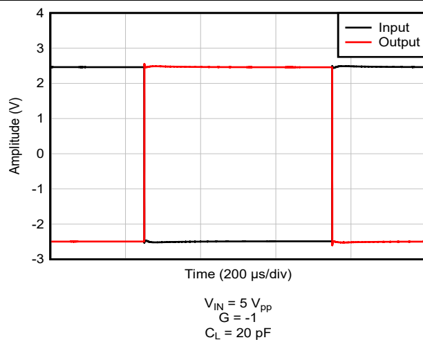
Figure 5-47. Large-Signal Step Response
