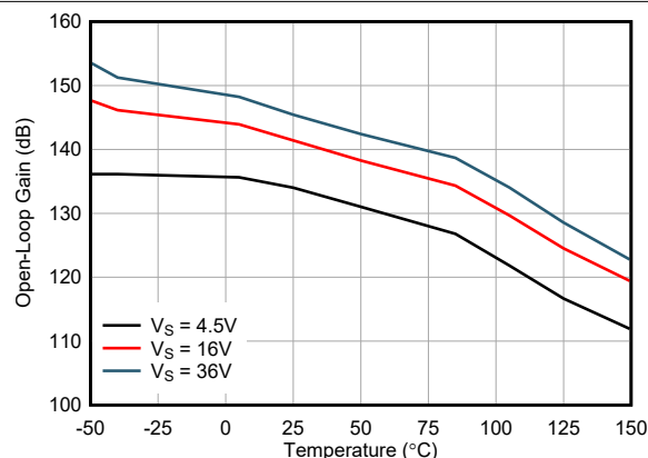
Figure 5-52. Open-Loop Gain vs Temperature
