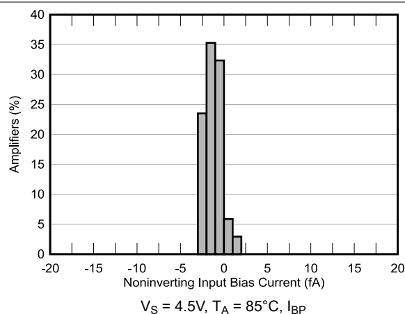
Figure 5-2. Input Bias Current Production Distribution
