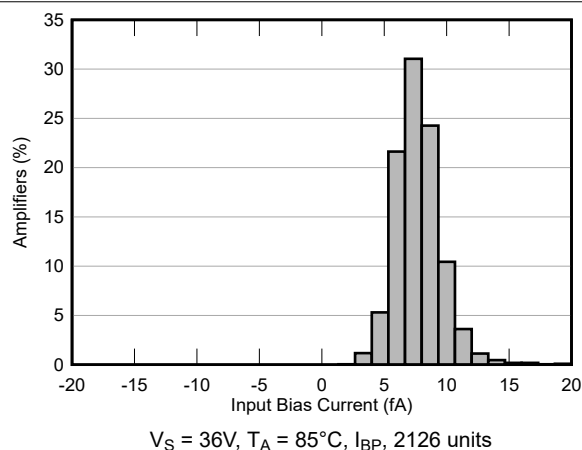
Figure 5-6. Input Bias Current Production Distribution
