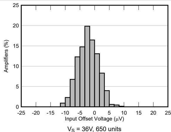
Figure 5-11. Offset Voltage Production Distribution
