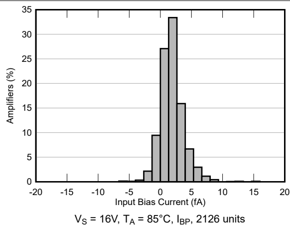
Figure 5-4. Input Bias Current Production Distribution
