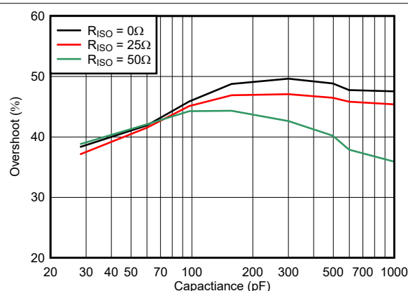
Figure 5-54. Small-Signal Overshoot vs Capacitive Load
