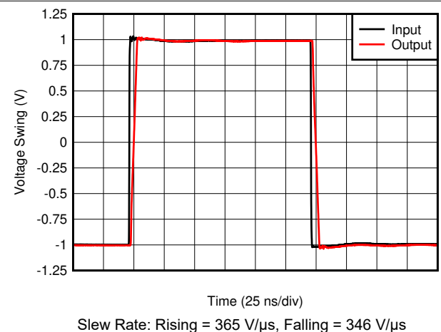
Figure 7-18. Large-Signal Transient Response
