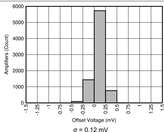
Figure 7-35. Offset Voltage Distribution
