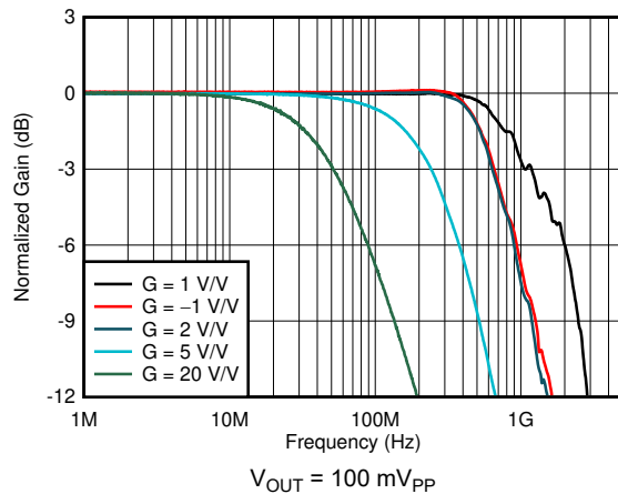
Figure 7-1. Small-Signal Response vs Gain
