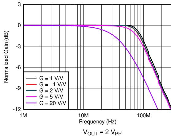
Figure 7-3. Large-Signal Response vs Gain
