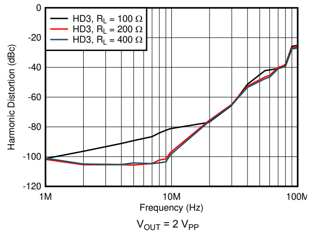
Figure 7-14. Harmonic Distortion (HD3) vs Load
