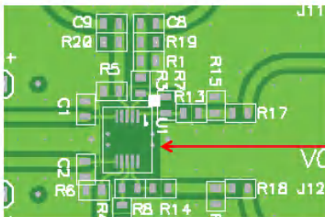
Figure 11-1. Top Layer
