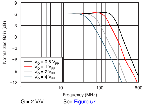
Figure 32. Noninverting Large-Signal Frequency Response
