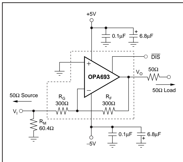
Figure 3. DC-Coupled, G = -1\text{V/V} , Bipolar-Supply Specification and Test Circuit.
