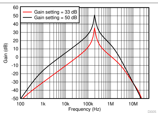
Figure 9-11. Hi-Z, High-Gain Front-End Circuit Gain vs Frequency
