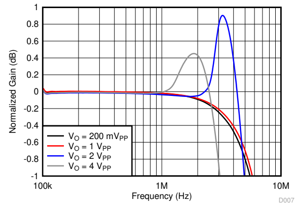
Figure 7-8. Large-Signal Response Flatness vs Frequency
