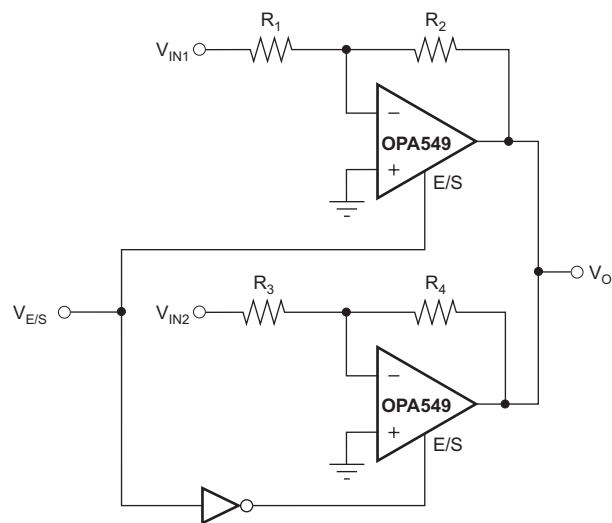
Figure 14. Switched Amplifier
