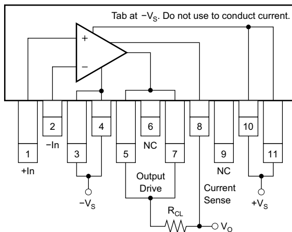
Pin Functions
