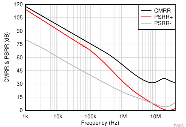
Figure 5-20. CMRR and PSRR vs Frequency
