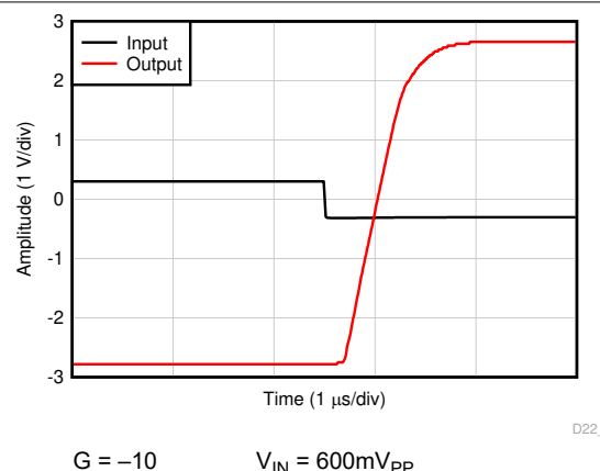
Figure 6-42. Overload Recovery
