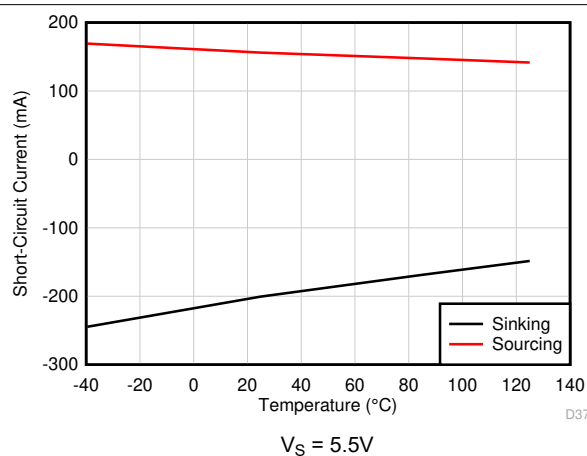
Figure 6-51. Short-Circuit Current vs Temperature
