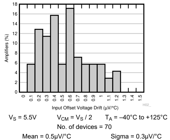
Figure 6-2. Offset Voltage Drift Distribution Histogram
