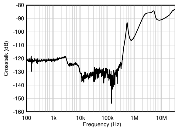
Figure 6-57. Channel Separation
