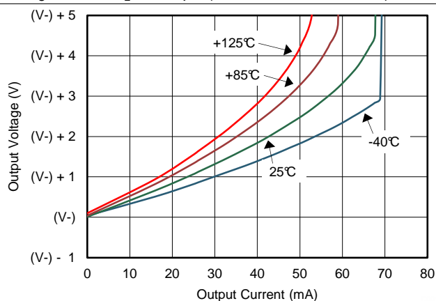
Figure 14. Output Voltage Swing from Negative Power Supply vs Output Current (Maximum Supply)
