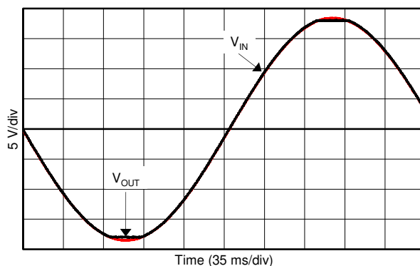
Figure 8-4. No Phase Reversal
