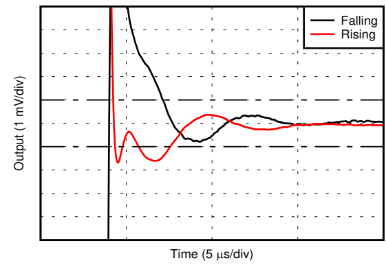
Figure 6-35. Settling Time
