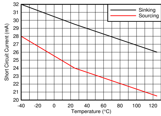
Figure 6-36. Short Circuit Current vs Temperature
