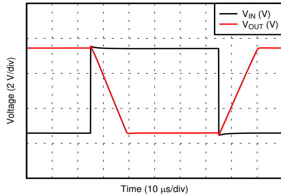
Figure 6-31. Small-Signal Step Response
