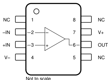
Figure 5-1. OPA186: D Package, 8-Pin SOIC (Top View)
