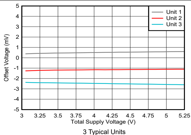
Figure 6-20. Offset Voltage vs Supply Voltage
