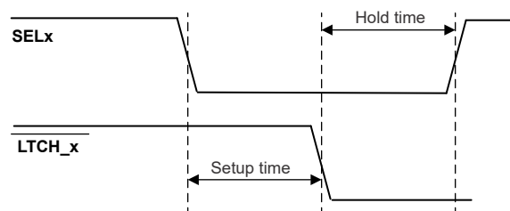
Figure 8-1. Timing Diagram
