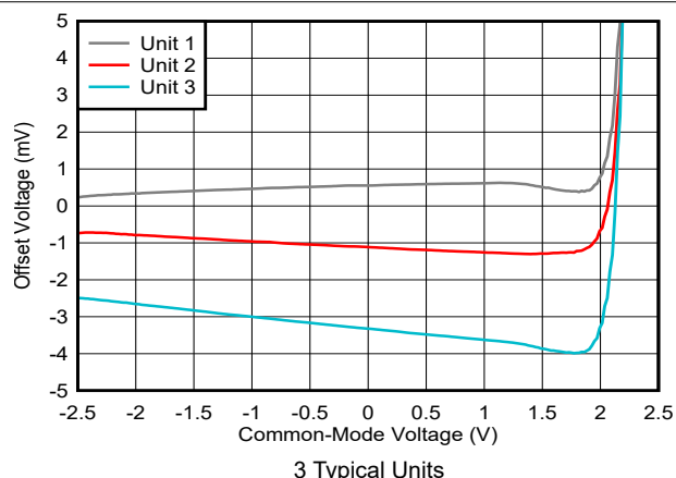
Figure 6-22. Offset Voltage vs Input Common-Mode Voltage
