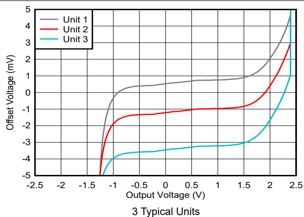
Figure 6-24. Offset Voltage vs Output Swing
