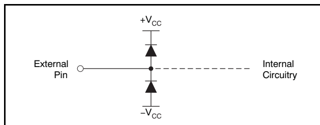
Figure 45. Internal ESD Protection
