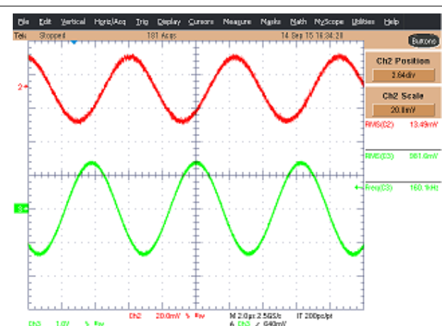
Figure 8-12. Gain Is -3 dB Above the Flat Gain at 160 kHz
