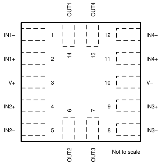
Figure 5-10. OPA990 RUC Package 14-Pin X2QFN With Exposed Thermal Pad Top View
