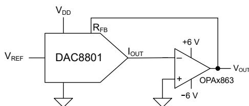
Figure 9-5. Variable Reference Generator Using MDAC and OPx863
