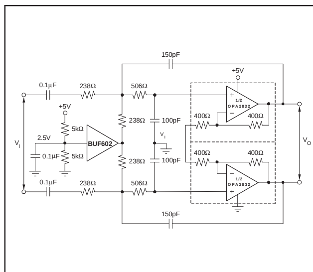
Figure 67. Single-Supply, 5MHz, 2nd-Order, Low-Pass Sallen-Key Filter
