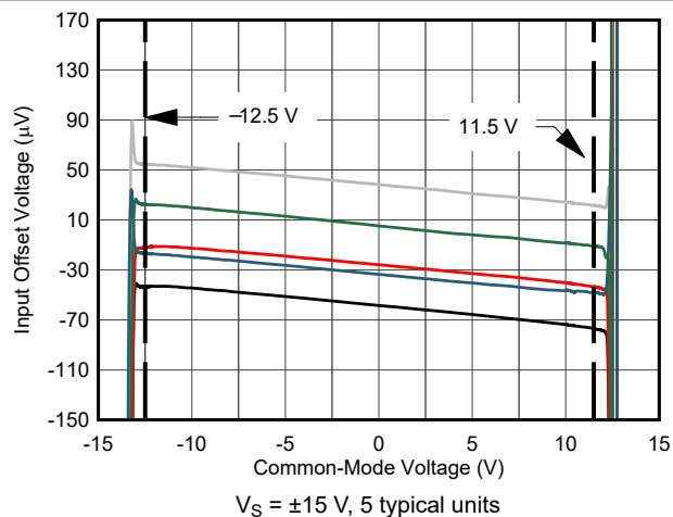
Figure 6-10. Offset Voltage vs Common-Mode Voltage
