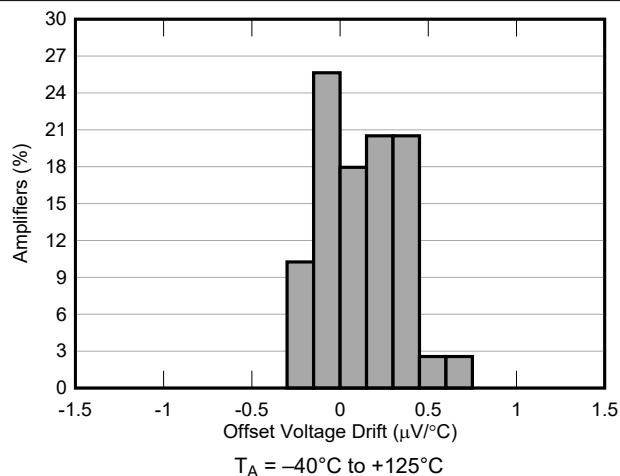
Figure 6-8. Offset Voltage Drift Production Distribution
