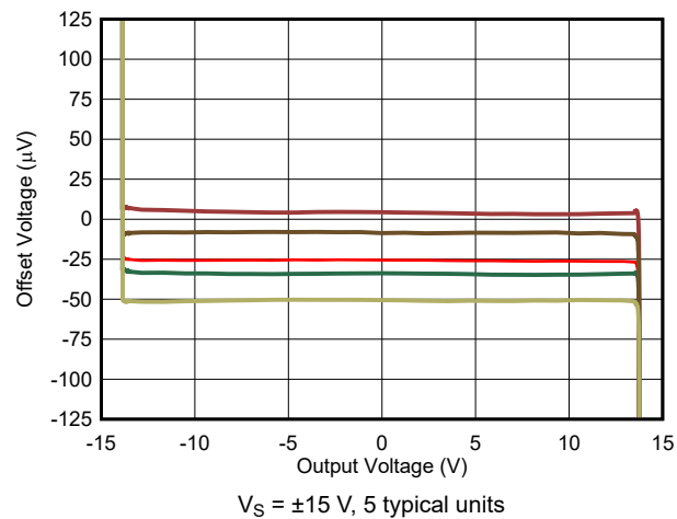
Figure 6-12. Offset Voltage vs Output Voltage
