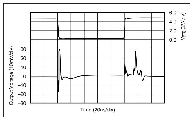
FIGURE 12. Disable/Enable Glitch.
