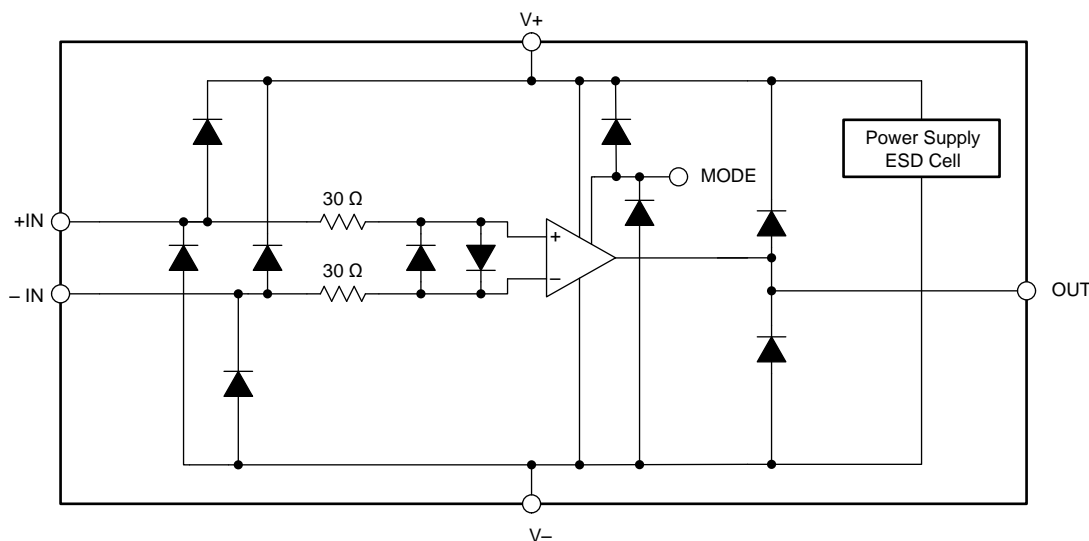
Figure 70. Simplified ESD Circuit
