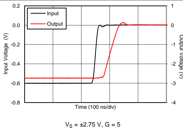
Figure 34. No Phase Reversal
