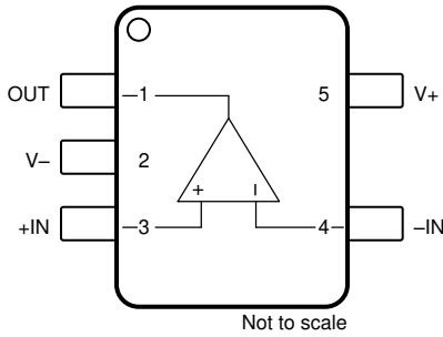
Figure 4-1. OPA383: DBV (Preview) Package, 5-Pin SOT-23 (Top View)
