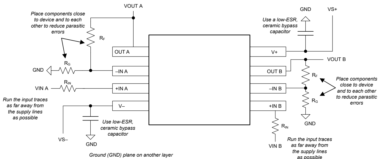
Figure 7-5. Layout Example
