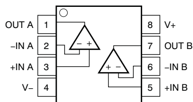
OPA2377-Q1: DGK Package 8-Pin VSSOP and SOIC Top View
