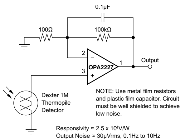
Figure 9. Long-Wavelength Infrared Detector Amplifier
