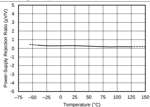
Figure 10. PSRR vs Temperature
