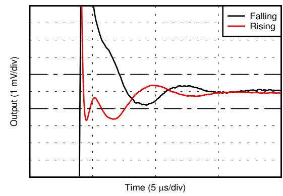
Figure 6-33. Large-Signal Step Response
