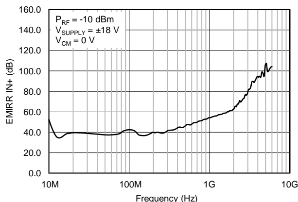
Figure 52. EMIRR Testing
