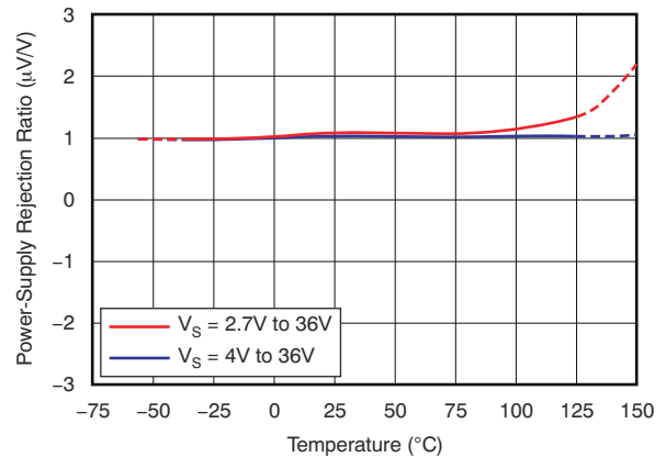
Figure 6-12. PSRR vs Temperature
