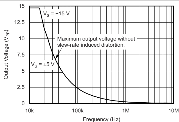
Figure 6-35. Maximum Output Voltage vs Frequency
