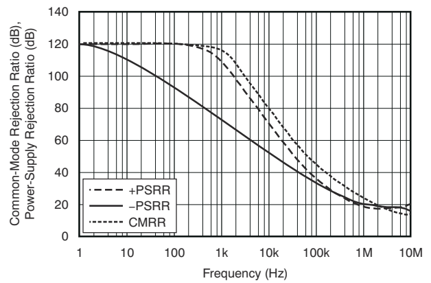
Figure 6-10. CMRR and PSRR vs Frequency (Referred-to Input)
