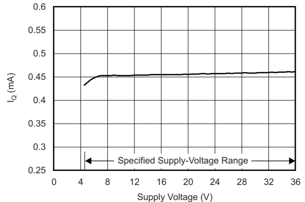
Figure 6-18. Quiescent Current vs Supply Voltage
