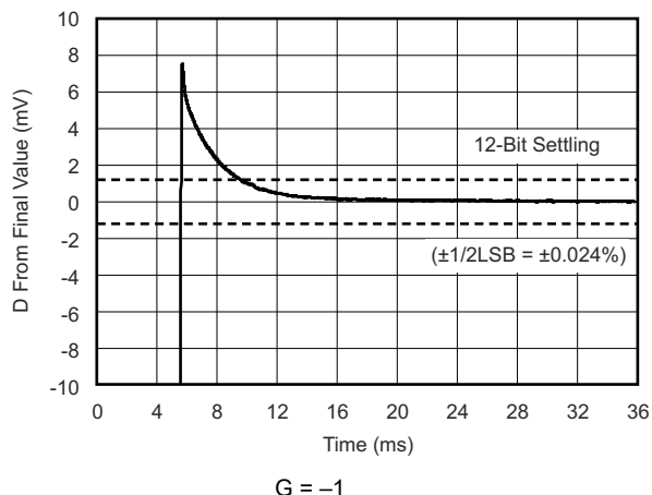
Figure 6-32. Large-Signal Settling Time (10-V Positive Step)
