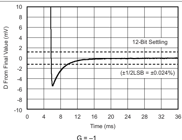
Figure 6-33. Large-Signal Settling Time (10-V Negative Step)
