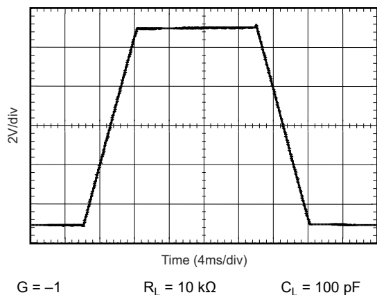
Figure 6-31. Large-Signal Step Response
