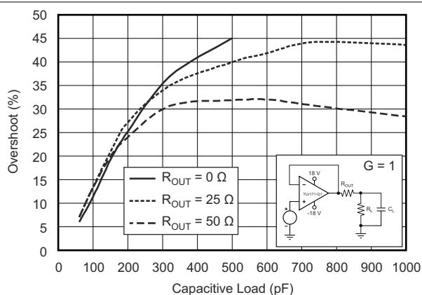
Figure 7-2. Small-Signal Overshoot versus Capacitive Load (100-mV Output Step)
