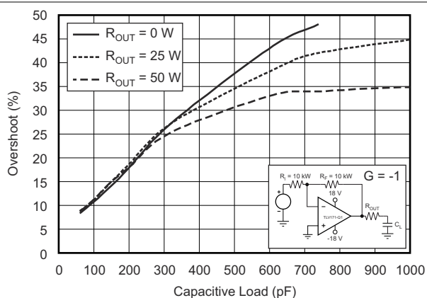
Figure 7-3. Small-Signal Overshoot versus Capacitive Load (100-mV Output Step)
