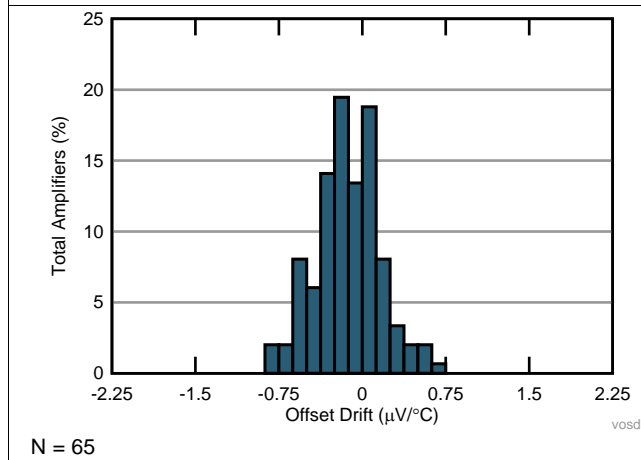
Figure 3. Offset Voltage Drift Distribution
